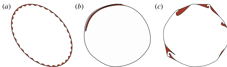
FIGURE 6. (Colour online) Cases of closed LAVD level sets benefiting from the relaxation of convexity to small convexity deficiency. The shaded area indicates the area difference between the level set and its convex hull. (a) A convex LAVD level set with a non-convex approximating polygon arising from discretization. (b) A closed LAVD level set with minor initial filamentation in the tangential direction. (c) A closed LAVD level set that is only convex after a filtering of smaller-scale vortices.
