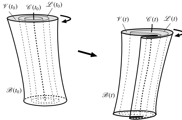
FIGURE 2. Initial and current positions of a rotationally coherent Lagrangian vortex \mathcal{V}(t) , a Lagrangian vortex boundary \mathcal{B}(t) and a Lagrangian vortex centre \mathcal{C}(t) . Also shown within \mathcal{V}(t) is a rotational LCS \mathcal{L}(t) , i.e. a material surface along which volume elements exhibit the same intrinsic dynamic rotation over the time interval [t_0, t_1] . As a consequence, \mathcal{V}(t) experiences only tangential material filamentation without global breakaway.
