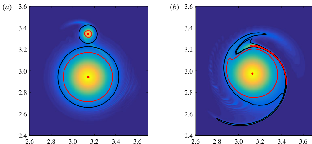
FIGURE 9. (a) Rotationally coherent Lagrangian vortex boundaries (red) at time t_0 = 0 in the vortex interaction example. Also shown are two circles (black) approximating the Eulerian vortex boundaries inferred at time t_0 from the vorticity distribution. The \text{LAVD}_0^{30}(\mathbf{x}_0) is shown in the background for reference. (b) The advected positions of the Lagrangian vortex boundaries and the two closed material curves at time t = 30 . The advected \text{LAVD} field \text{LAVD}_0^{30}(\mathbf{x}(30; 0, \mathbf{x}_0)) is shown in the background (see the online supplementary movie M2 for the complete advection sequence of the vortex boundaries).
