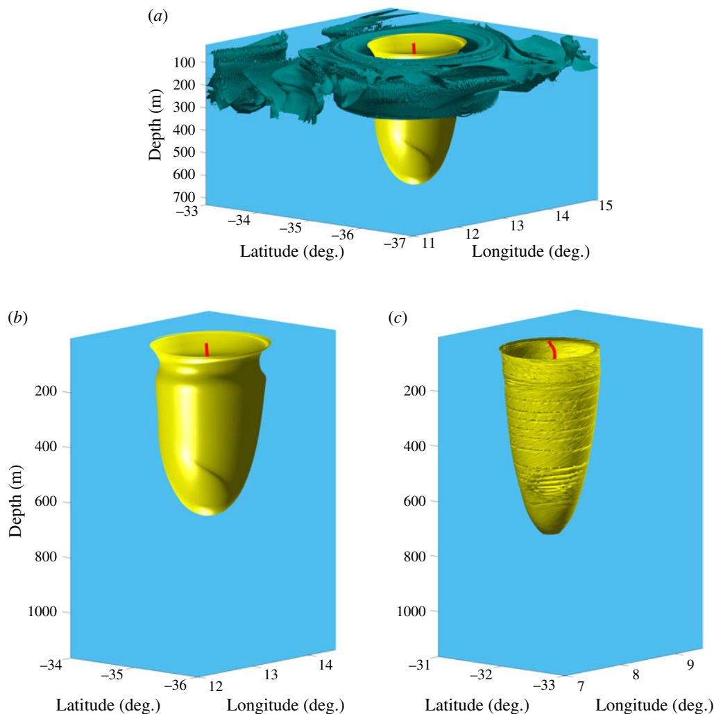
FIGURE 13. (a) Representative level surfaces of \text{LAVD}_{t_0+T}^{t_0}(\mathbf{x}_0) with t_0 = 15 May 2006 and T = 120 days. The yellow surface is extracted using Algorithm 2, marking the vortex boundary for a mesoscale rotationally coherent Lagrangian eddy, extending from 28 m down to 646 m in depth. The green surface is a nearby level surface of \text{LAVD}_{t_0+T}^{t_0}(\mathbf{x}_0) outside the Lagrangian vortex region. The red curve marks the coherent vortex centre, as defined in Definition 1. (b) Full view of the Lagrangian eddy boundary and its centre at the initial time t_0 . (c) The advected eddy boundary and vortex centre 120 days later, extending from 49 m down to 726 m below the surface (see the online supplementary movie M4 for the complete advection sequence of the eddy boundary).
