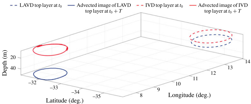
FIGURE 15. Initial top slices (dashed lines, at time t_0 = 15 May 2006) and their advected positions (solid lines, T = 120 days later) of the LAVD- and IVD-based rotationally coherent vortex boundaries.
