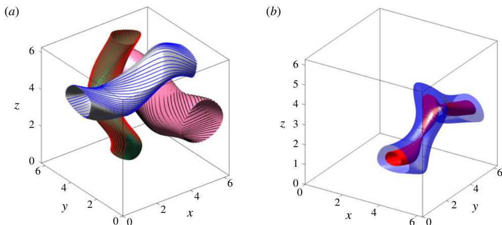
FIGURE 12. (a) Three representative rotationally coherent Lagrangian vortex boundaries in the ABC flow, obtained as outermost convex tubular level sets of \text{LAVD}_0^{50}(\mathbf{x}_0) . Black curves indicate trajectories launched on these boundaries. (b) Two representative \text{IVD}(\mathbf{x}) level surfaces (with blue denoting the rotationally coherent Eulerian vortex boundary) in the single Eulerian coherent vortex obtained from the IVD field for the ABC flow for the parameter values considered here.
