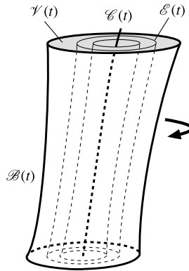
FIGURE 3. A rotationally coherent Eulerian vortex \mathcal{V}(t) , with boundary \mathcal{B}(t) and vortex centre \mathcal{C}(t) . Also shown within \mathcal{V}(t) is a rotational ECS \mathcal{E}(t) , i.e. a surface along which volume elements exhibit the same intrinsic dynamic rotation rate instantaneously at time t . No material coherence is guaranteed for the Eulerian vortex \mathcal{V}(t) under passive advection.
