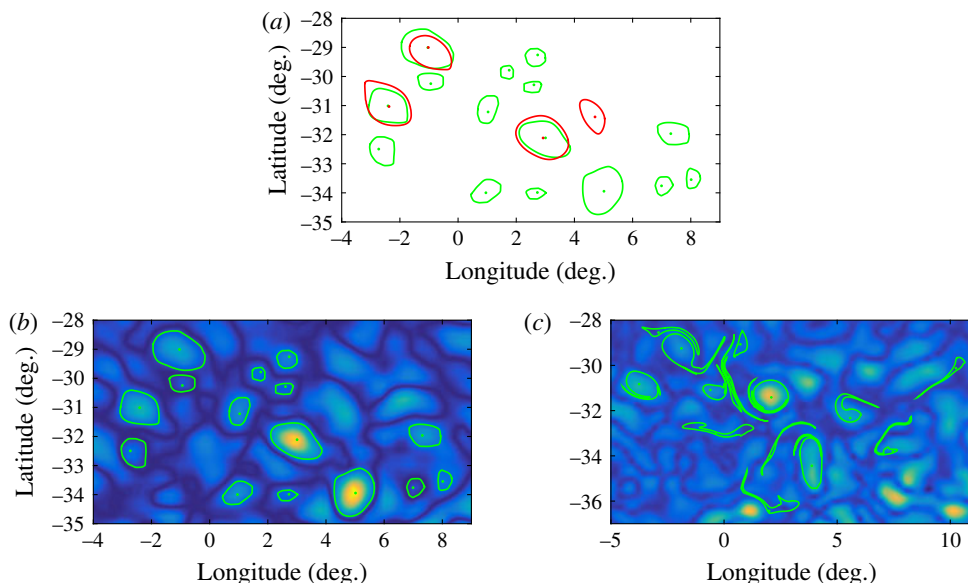
FIGURE 11. (a) Lagrangian (red) and Eulerian (green) rotationally coherent vortices at time t_0 in the satellite altimetry example. (b) Rotationally coherent Eulerian vortex boundaries and centres at time t_0 , with the \text{IVD}(\mathbf{x}, t_0) field shown in the background. (c) The same objects advected passively to the final time t_1 = t_0 + T , with \text{IVD}(\mathbf{x}, t_1) shown in the background.
