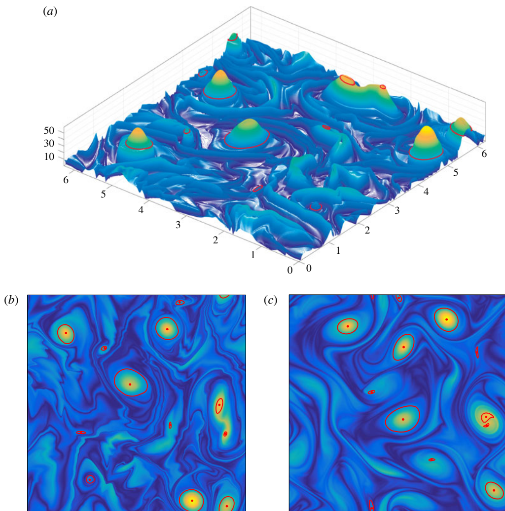
FIGURE 7. (a) Three-dimensional contour plot of \text{LAVD}_0^{50}(\mathbf{x}_0) . Lagrangian vortex boundaries (outermost rotational LCSs) extracted from Algorithm 1 are shown in red. (b) Vortex boundaries shown in the flow domain at initial time t=0 . The contour plot of \text{LAVD}_0^{50}(\mathbf{x}_0) is shown in the background for reference. (c) Advected Lagrangian vortex boundaries at the final time t_1 = 50 (see the online supplementary movie M1 for the complete advection sequence of the vortex boundaries).
