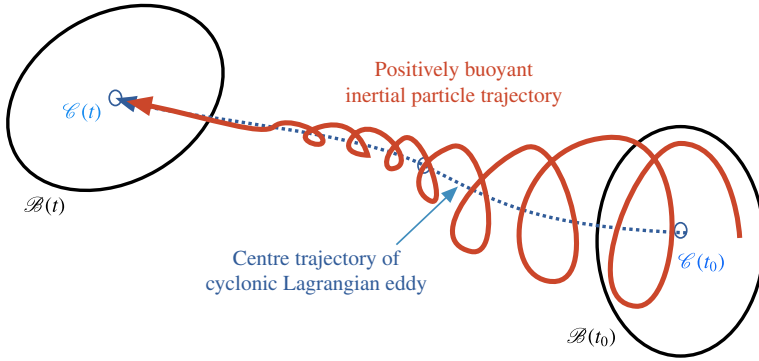
FIGURE 5. By Theorem 2, cyclonic Lagrangian eddy centres evolving from LAVD maxima act as observed attractors for small positively buoyant particles, such as drifters and floating debris.
