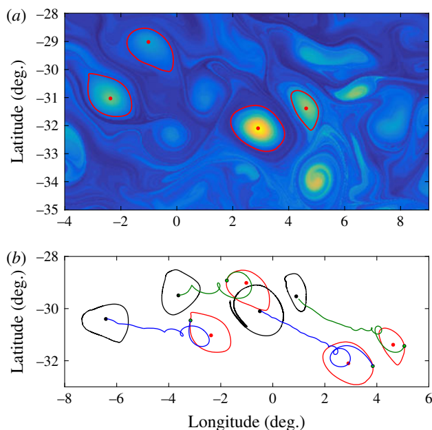
FIGURE 10. (a) Rotationally coherent Lagrangian vortices at time t_0 = 11 November 2006, identified from Algorithm 1 using the contours of \text{LAVD}_{t_0}^{t_0+T}(\mathbf{x}_0) with T = 90 days. The contour plot of \text{LAVD}_{t_0}^{t_0+T}(\mathbf{x}_0) is shown in the background for reference. (b) Initial (red) and final (black) positions of the Lagrangian vortex boundaries at time t_0 + T , along with representative inertial particle trajectories. Heavy particles (blue) converge to the centres of anticyclonic (clockwise) eddies. Light particles (green) converge to the centres of cyclonic (clockwise) eddies. Here, \delta_{\text{heavy}} = 0.99 , \delta_{\text{light}} = 1.01 , r_0 = 1 m. (See the online supplementary movie M3 for the complete advection sequence of the vortex boundaries and the inertial particles.)
