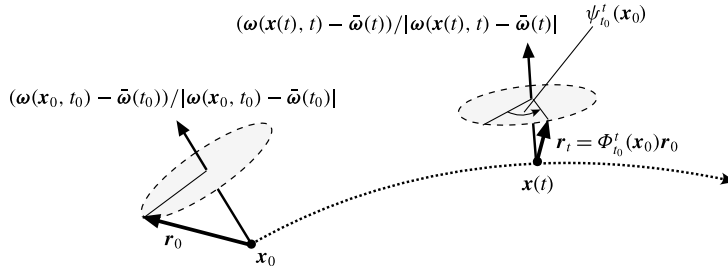
FIGURE 1. The geometry of the intrinsic rotation angle \psi_{t_0}^t(\mathbf{x}_0) along a material trajectory \mathbf{x}(t) in a three-dimensional deforming continuum.
