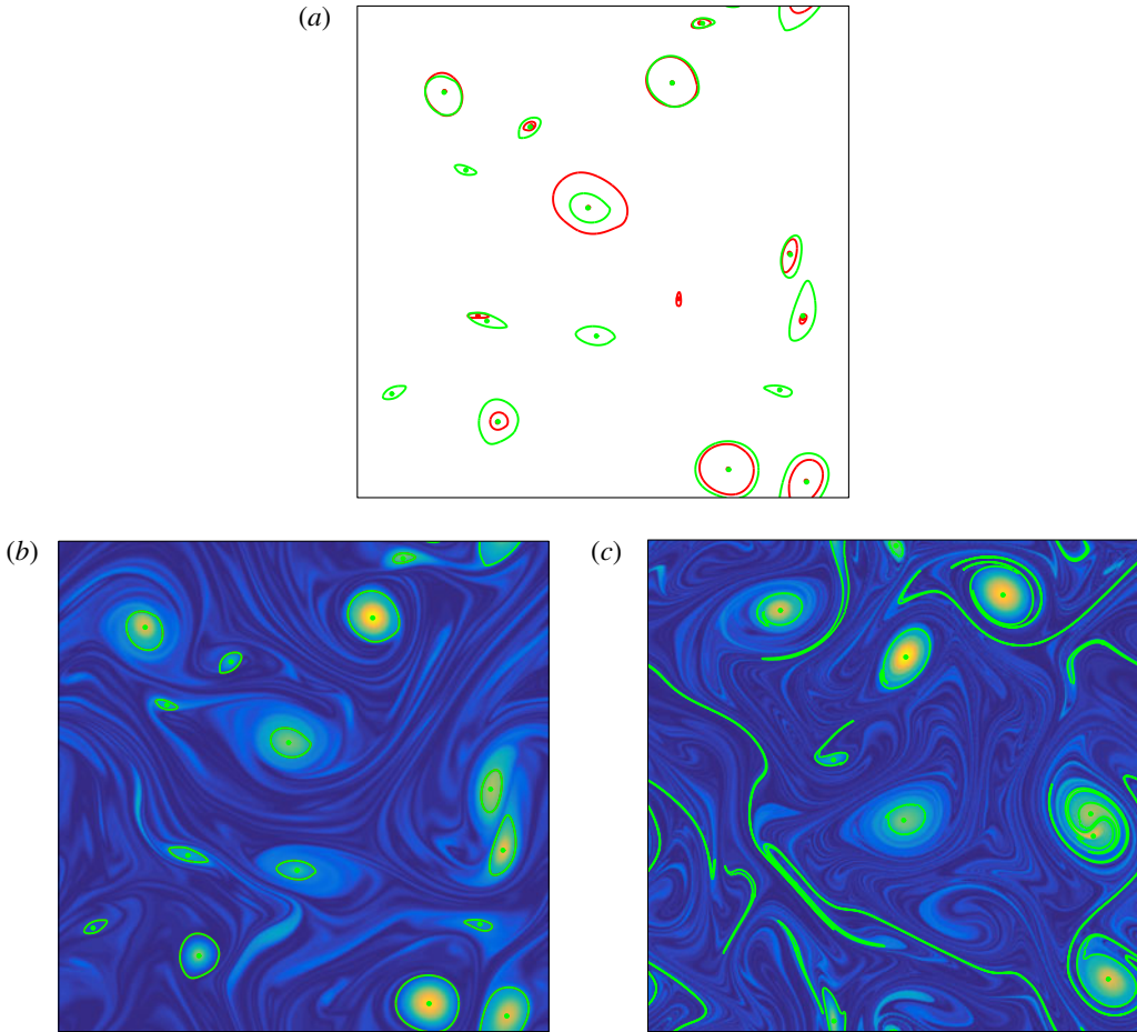
FIGURE 8. (a) Lagrangian (red) and Eulerian (green) rotationally coherent vortices at time t_0 in the two-dimensional turbulence example. (b) Rotationally coherent Eulerian vortex boundaries and centres at time t_0 , with the \text{IVD}(\mathbf{x}, t_0) field shown in the background. (c) The same objects advected passively to the final time t_1 = 50 , with \text{IVD}(\mathbf{x}, t_1) shown in the background.
