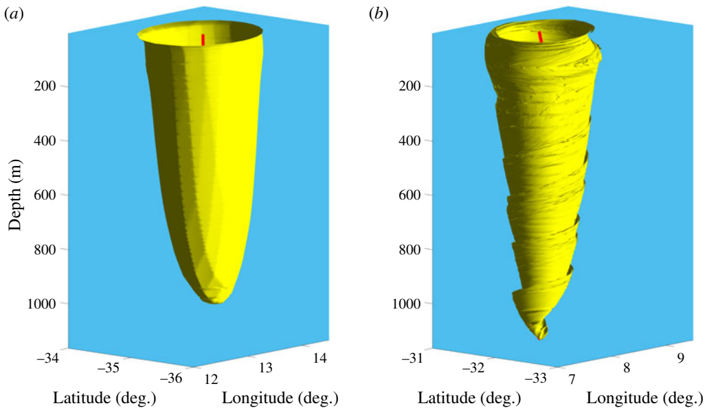
FIGURE 14. (a) The rotationally coherent Eulerian counterpart of the Lagrangian eddy shown in figure 13(a), ranging from 7 m down to 1007 m below the sea surface. (b) The materially advected position of the Eulerian eddy 120 days later, ranging from 15 to 1163 m below the sea surface (see the online supplementary movie M5 for the complete advection sequence of the eddy boundary).
