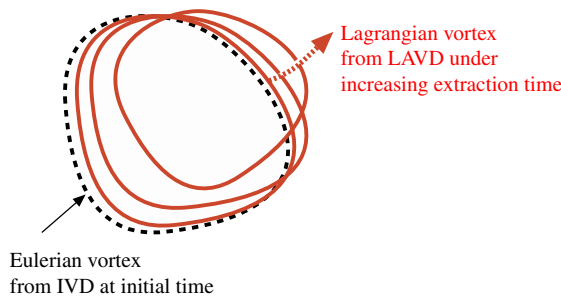
FIGURE 4. A rotationally coherent Eulerian vortex is the limit of a rotationally coherent Lagrangian vortex under vanishing extraction time (i.e. integration time).
