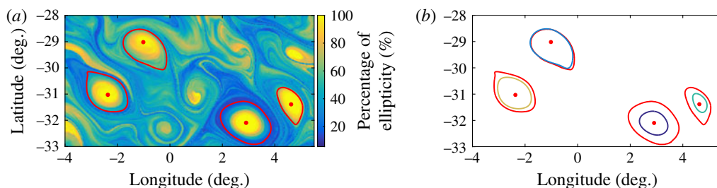
FIGURE 16. (a) The ellipticity-time field \tau_e(t_1, t_0, \mathbf{x}_0) for the Agulhas leakage data set of § 10.5 with t_0 = 11 November 2006 and t_1 = t_0 + 90 days. Rotationally coherent Lagrangian vortex boundaries (red) are superimposed for reference. (b) Geodesic vortex boundaries at time t_0 for the same data set, with the LAVD-based vortex boundaries (red) superimposed.
