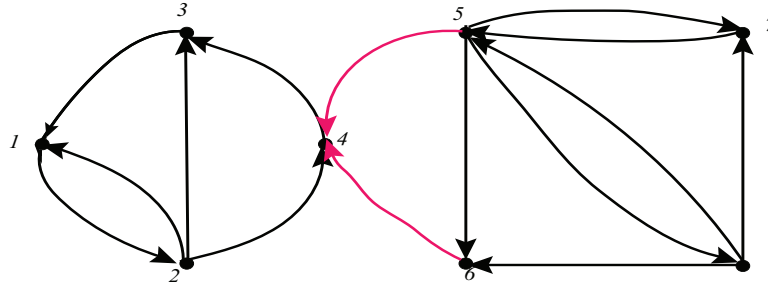
Figure 4.3. Another HMC with a single irreducible subset.
