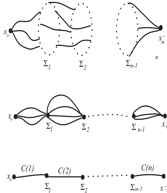
Figure 4.7. Shorting an infinite electric network inside spheres.
