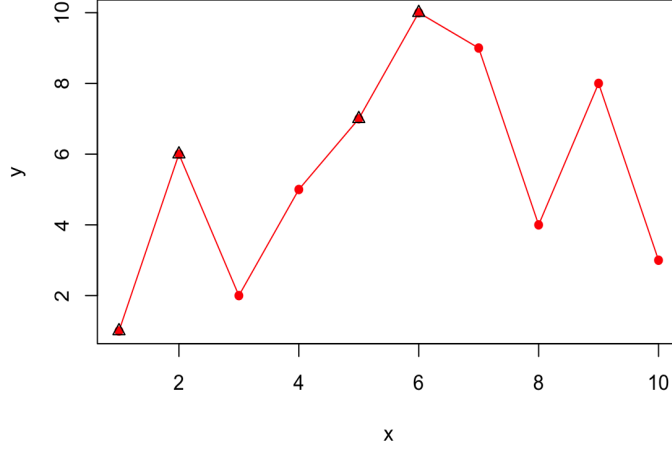
Figure 4.5. A zig-zag depicting a permutation and its leading points, marked with a triangle. The zig-zag connects the points (j, \varphi(j)) , 1 \leq j \leq n , by line segments.
