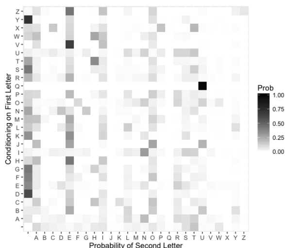
Figure 4.9. Moby Dick Transition Matrix
