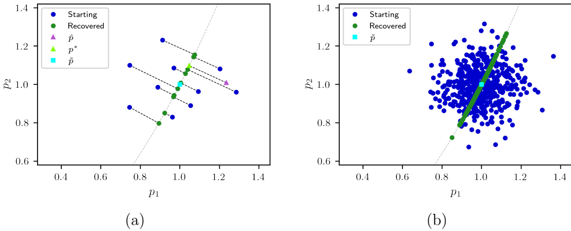
Figure 5: (a) Illustration of recovering parameters for various perturbations including the example summarized in Table S8; (b) Illustration using 500 samples
